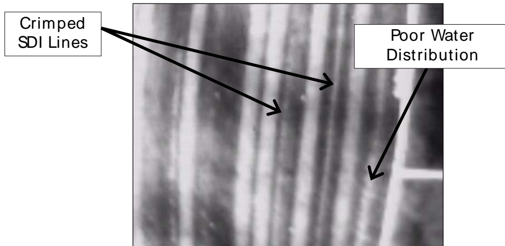
Figure 2. Thermal infrared image showing crimped SDI tape and an area of poor water distribution.
