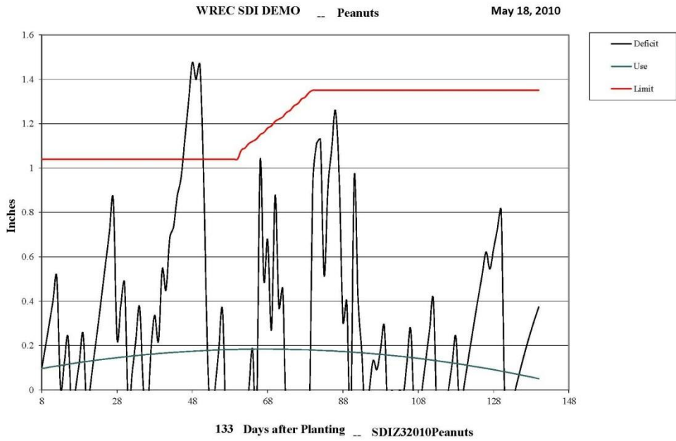
Figure 4B - 2010 SDI Peanut Demo Season IRR Soil Moisture Deficit
