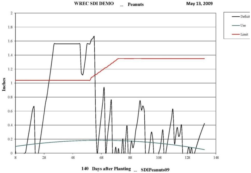
Figure 2A - 2009 SDI Peanut Demo Season RAINFALL-ONLY Soil Moisture Deficit
