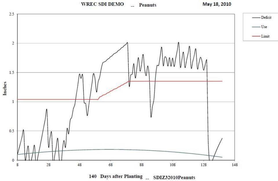
Figure 4A - 2010 SDI Peanut Demo Season RAINFALL-ONLY Soil Moisture Deficit
